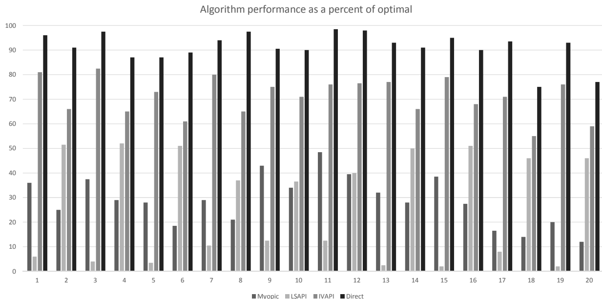
Figure 6: The performance of a series of approximation algorithms relative to the optimal solution for 20 benchmark storage problems. These include: a myopic policy, a basic form of least squares approximate policy iteration, LSAPI with instrumental variables, and direct policy search using the same structure for the policy (from Scott et al. (2013)).
