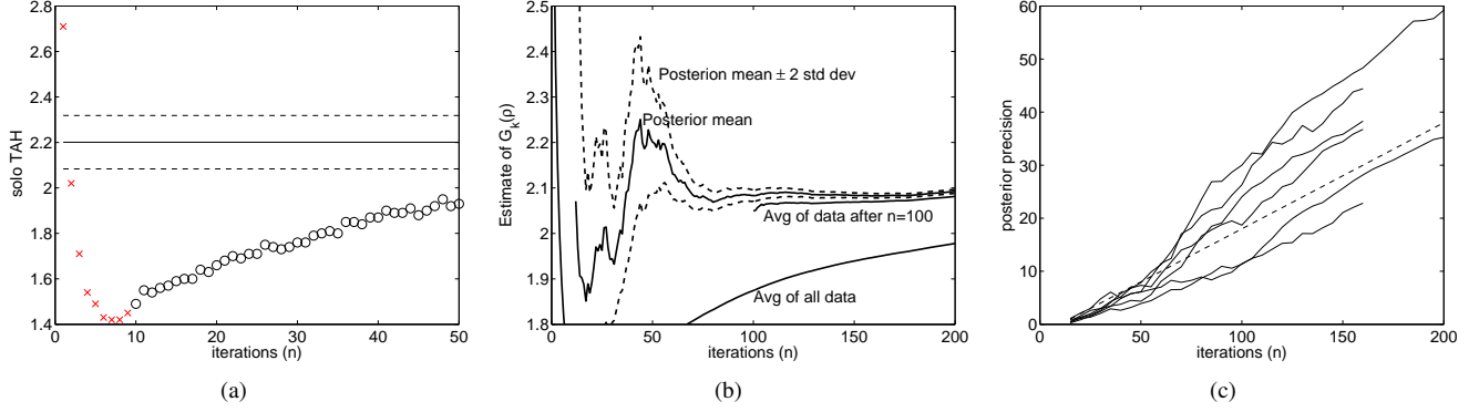
Figure 2: Figure 2(a) shows the posterior mean and standard deviation resulting from a Bayesian analysis of the first 50 of the iterations in Figure 1. Figure 2(b) displays estimates from the three different estimation methods discussed in the text as a function of how many iterations the method observes. In Figure 2(c), the solid lines show precision of the posterior on G_k(\rho) as a function of the number of iterations for several different values of k and \rho . The dotted line shows a linear fit of 0.2(n - n_0) , where n_0 = 10 .
